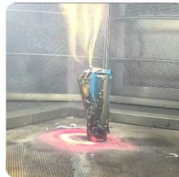
Battery Burn-resistant Tester
