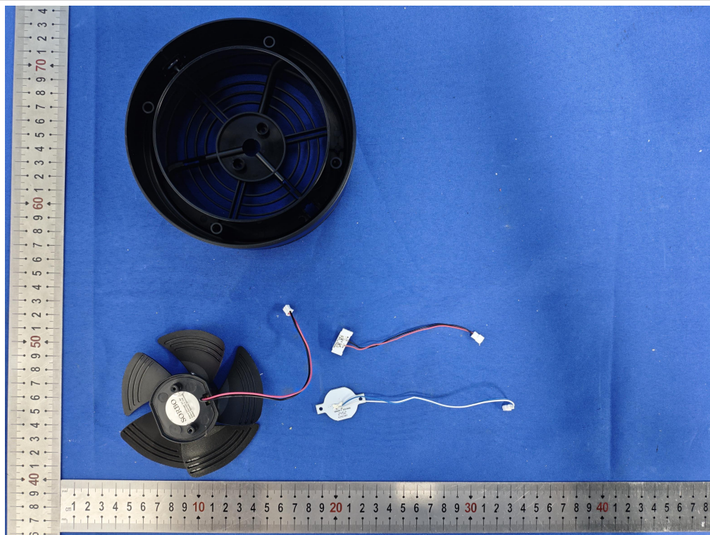
Photo 12 Internal view
